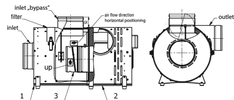
Fig 4.a. Construction
