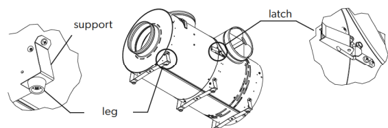
Fig 4.b. Construction
