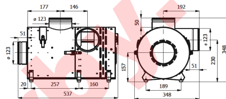
Fig 3.a. Dimensions BANANeco1-II
