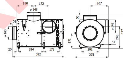
Fig 3.b. Dimensions BANANeco2-II
