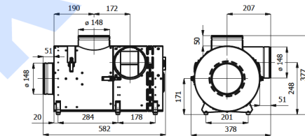
Fig 3.b. Dimensions BANANeco2-II
